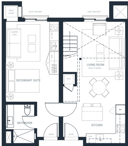
LOWER LEVEL
